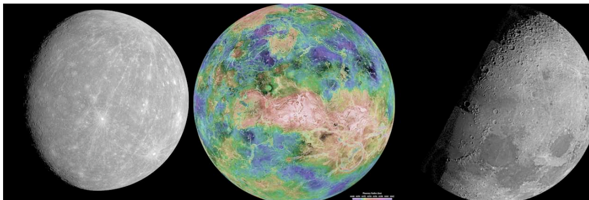
FIGURE 5.1 Mercury, Venus, and the Moon are essential to understanding how terrestrial planets form and change with time. SOURCE: Mercury : NASA/JPL; Venus : NASA/JPL/USGS; Moon : NASA/JPL.
