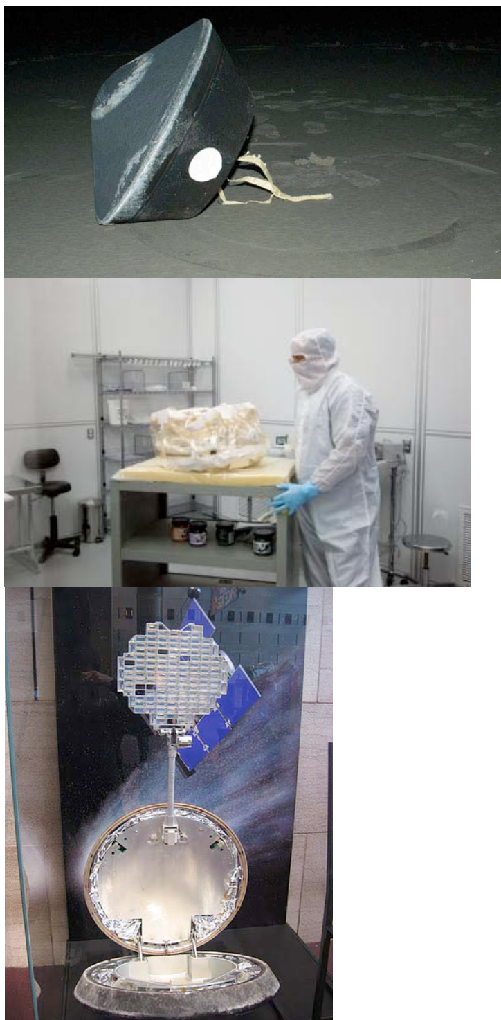
FIGURE 1.10 From a comet, to the desert, to the laboratory, to the Smithsonian—the Stardust mission encountered the comet Wild 2 in January 2004, and returned samples to Earth in January 2006 ( top ). The samples are still being examined but have provided new understandings of our solar system. The capsule now resides in the National Air and Space Museum ( bottom ). SOURCE: Top, middle: NASA/JPL. Bottom: Smithsonian National Air and Space Museum.
