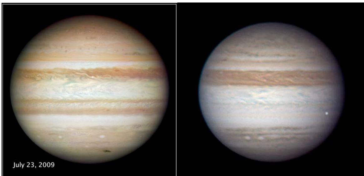
FIGURE 7.2 Left: This Hubble image of Jupiter shows the aftermath of an impact in 2009. The collision created a debris field the size of the Pacific Ocean (dark region on lower right), similar to the sites created by the impacts of the Shoemaker-Levy 9 fragments in 1994. Right: Yet another impact occurred on Jupiter in 2010, this time seen only during its fireball phase (bright spot on right edge of planet). Two different amateur astronomers captured the meteor on video, but the impact left no detectable trace in the atmosphere even in observations with the world’s most powerful telescopes, including Hubble and Gemini. SOURCE: Left: Courtesy NASA, ESA, M. H. Wong, H. B. Hammel, and the Hubble Impact Team. Right: Courtesy of Anthony Wesley.
